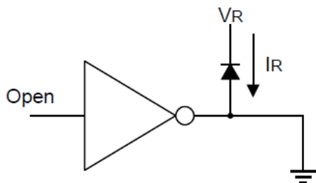
Figure 7 IR Test Circuit
