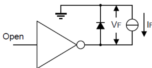
Figure 8 VF Test Circuit
