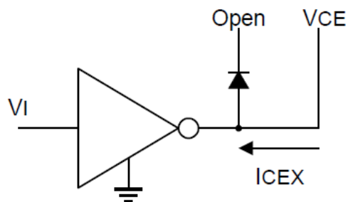
Figure 2 ICEX Test Circuit
