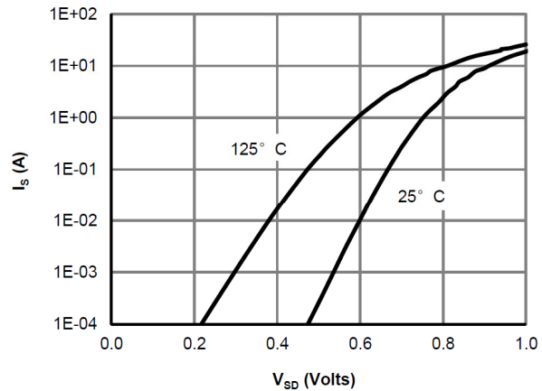
Figure 6: Body-Diode Characteristics
