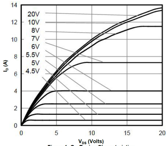
Figure 1: On-Region Characteristics
