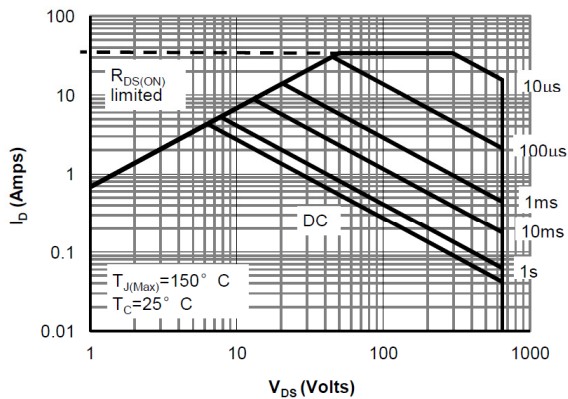
Figure 11: Maximum Forward Biased Safe Operating Area
