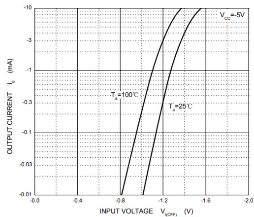
Figure 2: OFF Characteristics
