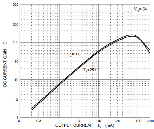
Figure 3: G_I — I_O
