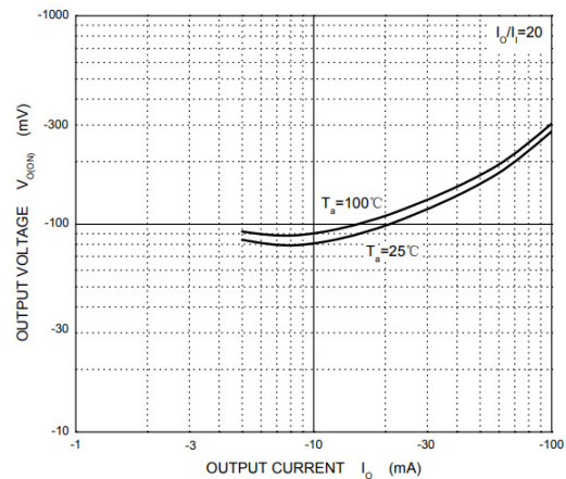
Figure 4: V_{O(ON)} — I_O
