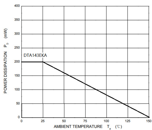
Figure 6: P_D — T_a
