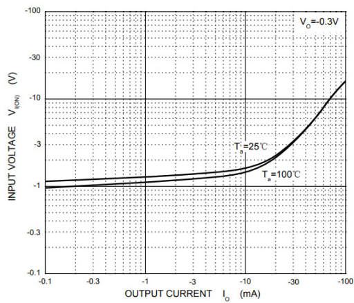
Figure 1: ON Characteristics
