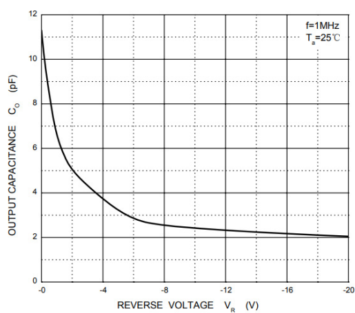
Figure 5: C_O — V_R
